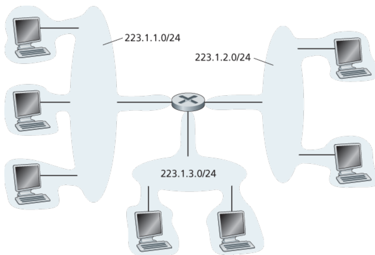
Figure 4.19 Subnet addresses
