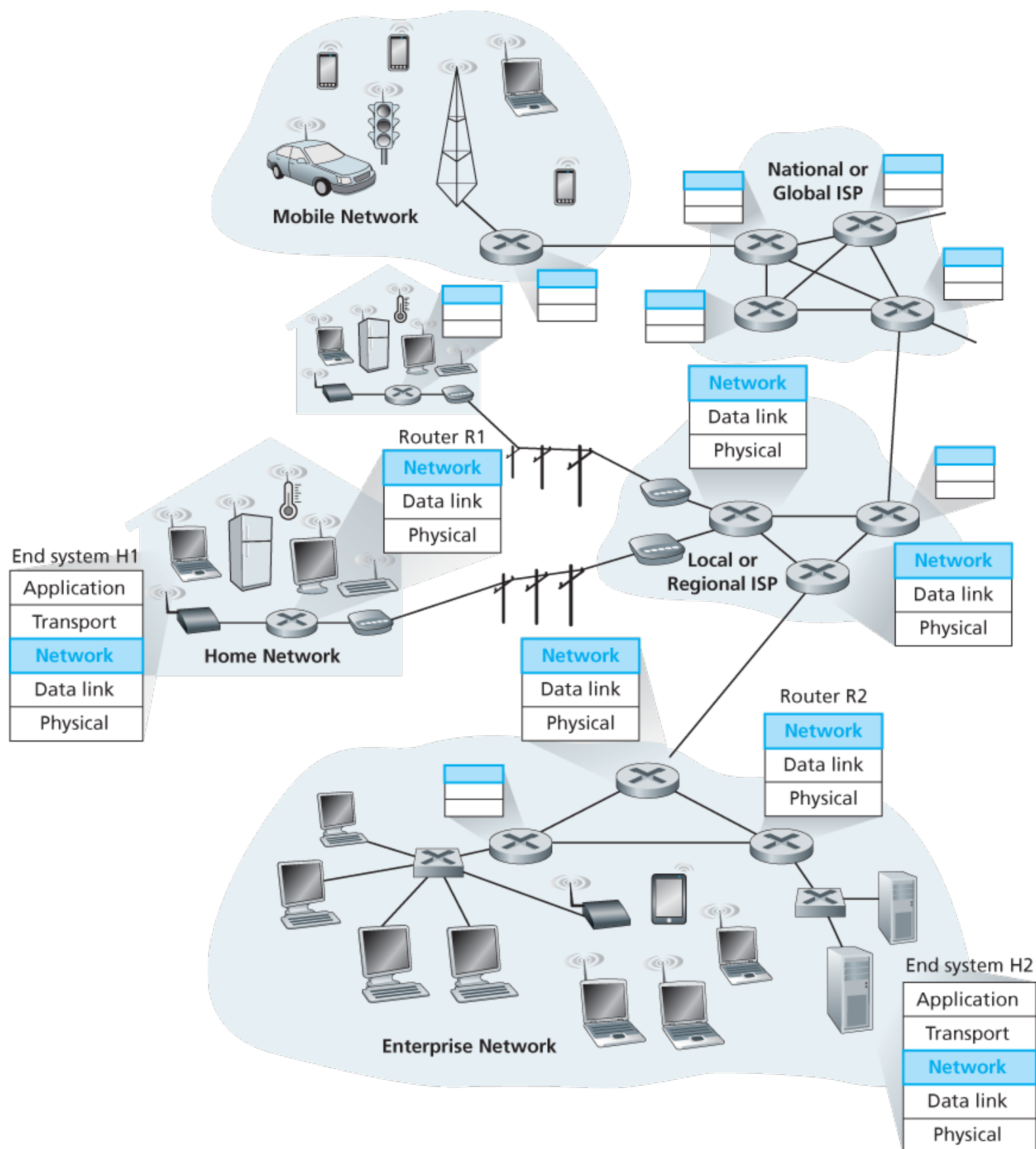
Figure 4.1 The network layer
