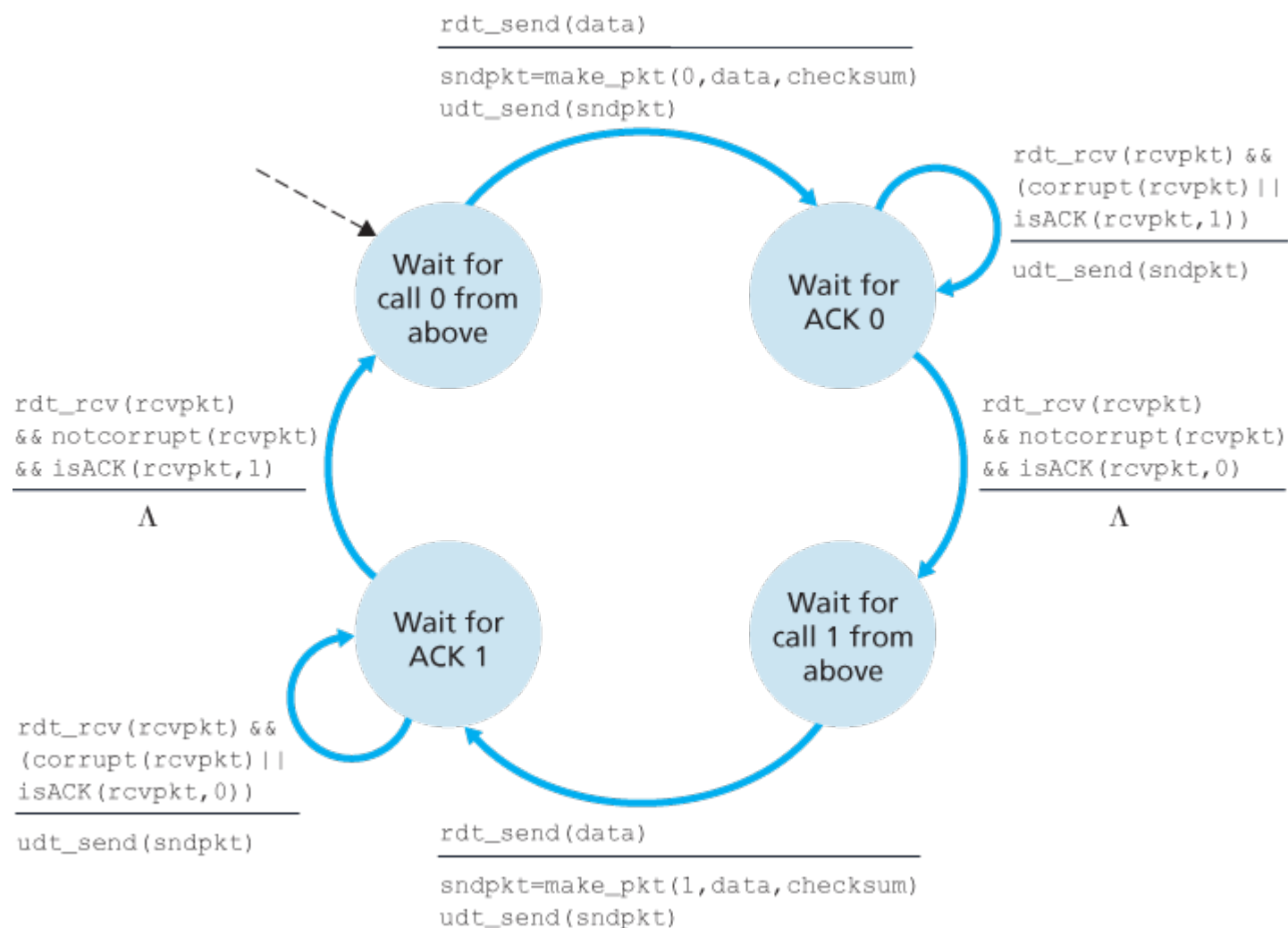
Figure 3.13 rdt2.2 sender
