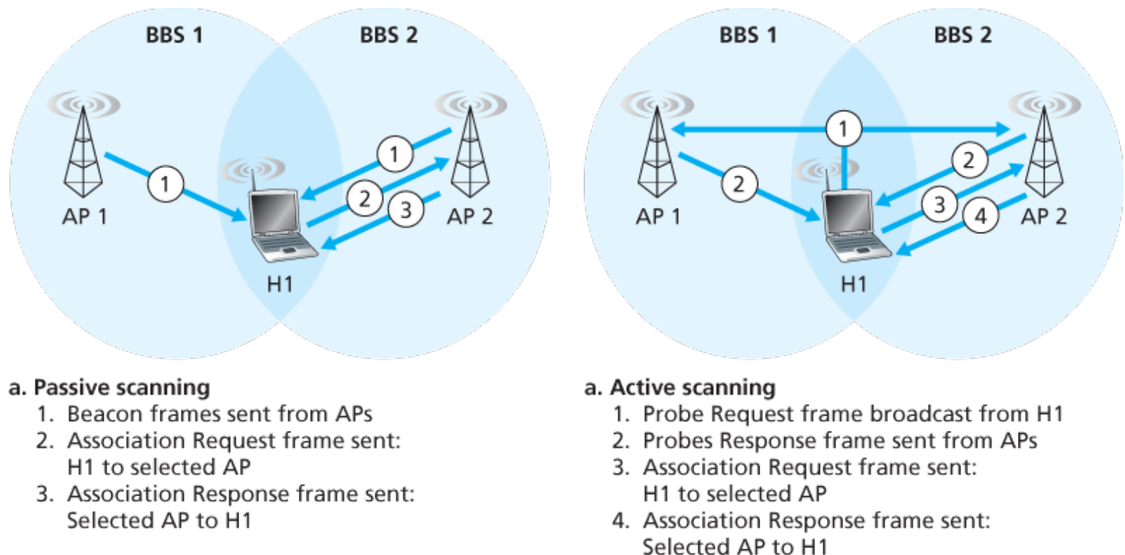
Figure 7.9 Active and passive scanning for access points
