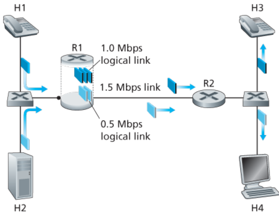
Figure 9.13 Logical isolation of audio and HTTP traffic classes
