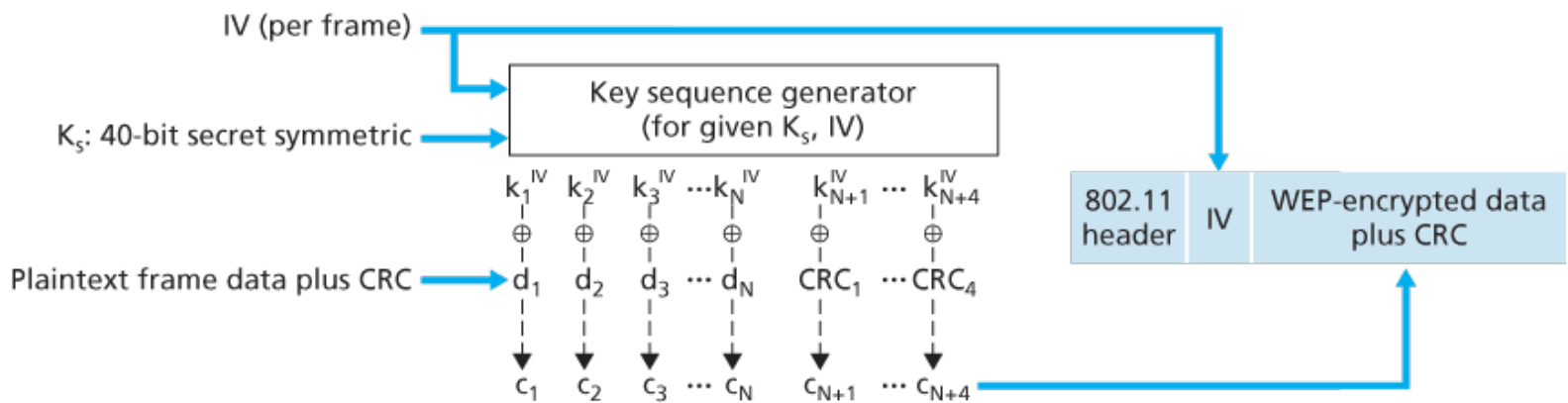
Figure 8.30 802.11 WEP protocol
