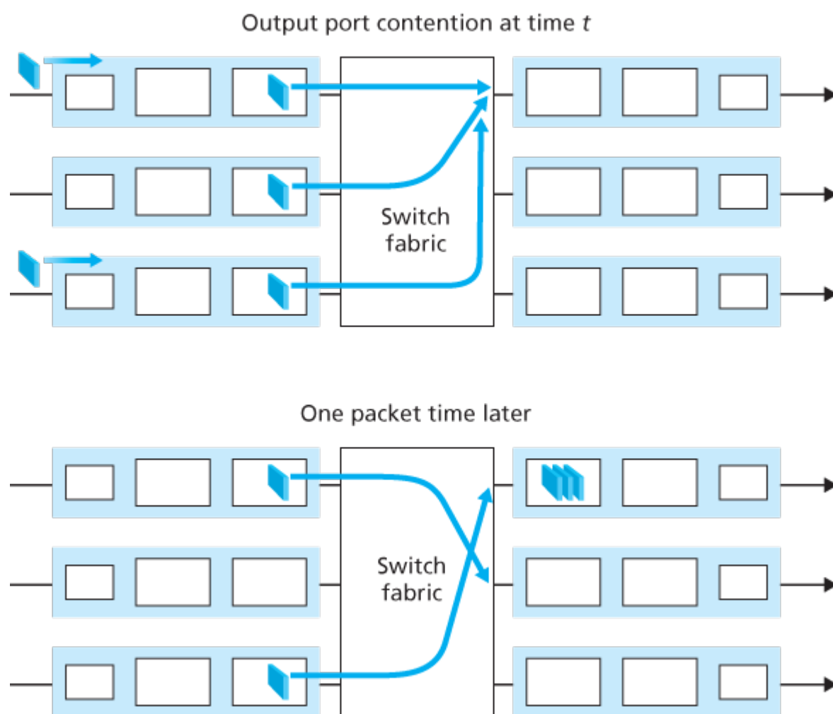
Figure 4.9 Output port queuing
