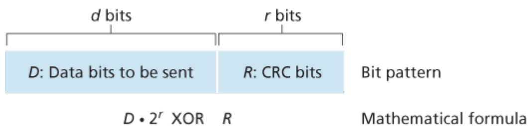
Figure 6.6 CRC
